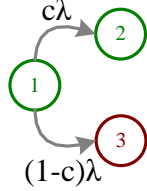
Fig. 18. Incorporating FDIR effectiveness using fault coverage
