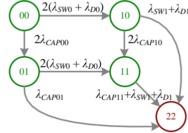
Fig. 21. State-transition diagram of two-phase converter
