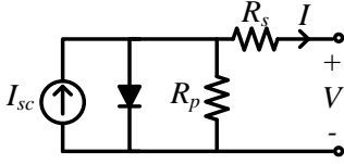
Fig. 2. Solar cell model
